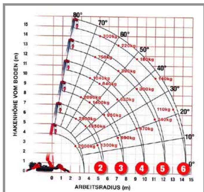
Unic URW 376
