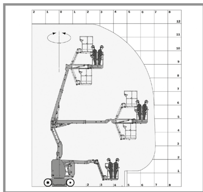
Manitou 120
