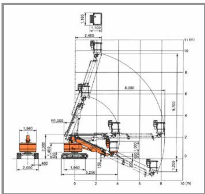
Hitachi HX 99 B
