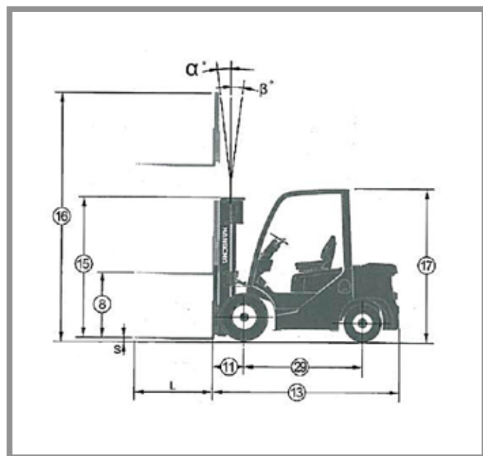
Hangcha XF FG35
