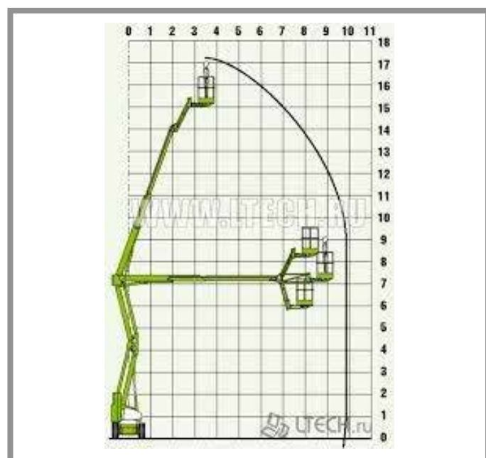
NIFTY 17M
