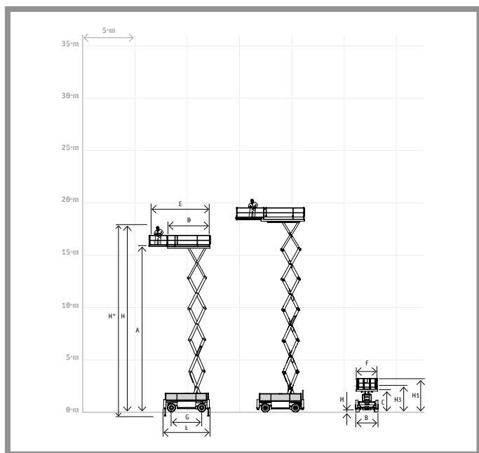
Holland Lift dl 22M
