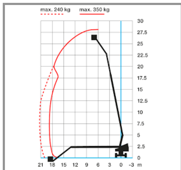
Manitou 280 TJ
