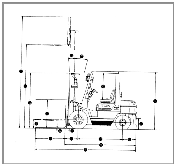
TCM Gastruck FG30N8T
