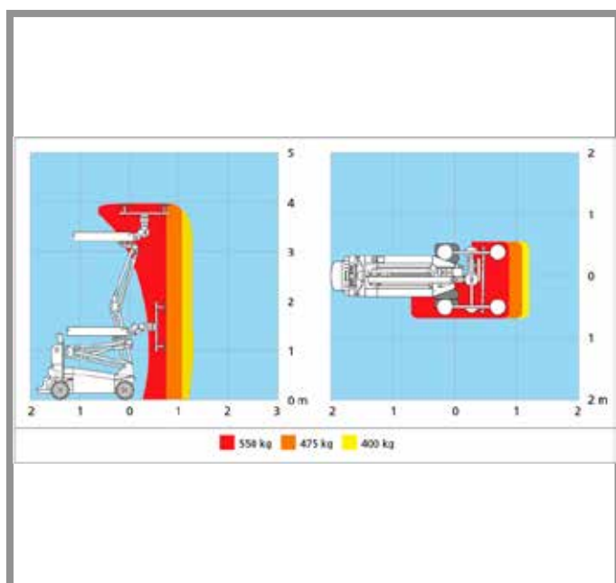
Glaslift 550 Terrain
