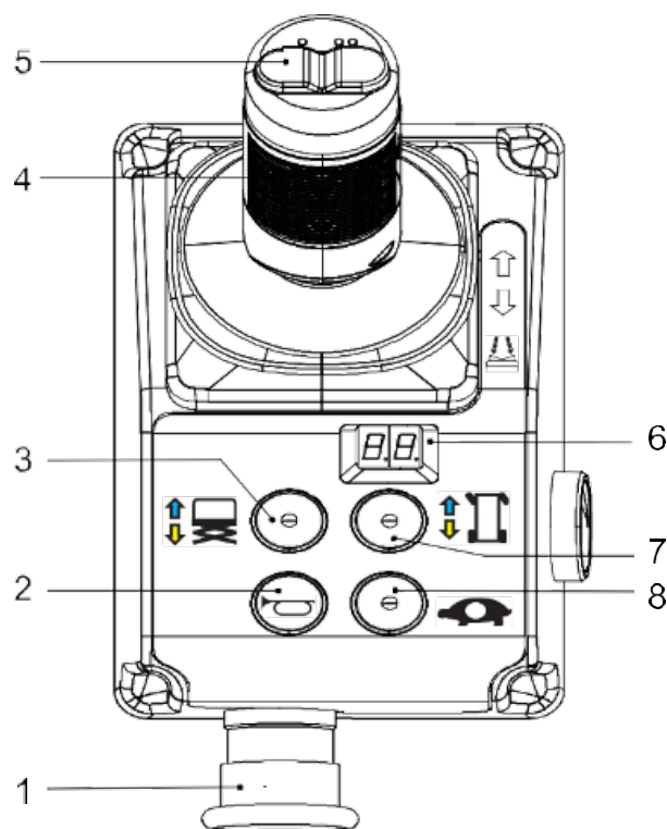
Figur 2-5 Platformsbetjeningspanel
