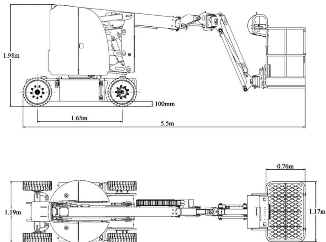
Figur 7-1 ZA10RJE Dimensioner I transport position
