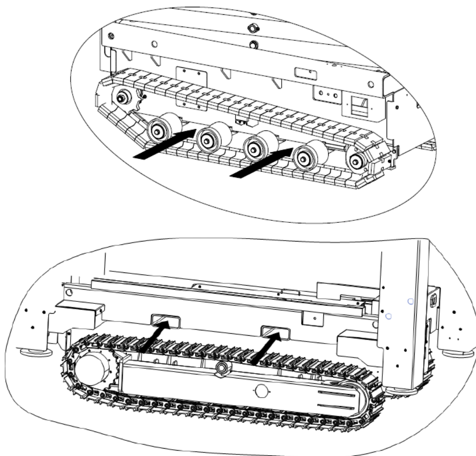
Figur 4-4 Trucklommer
